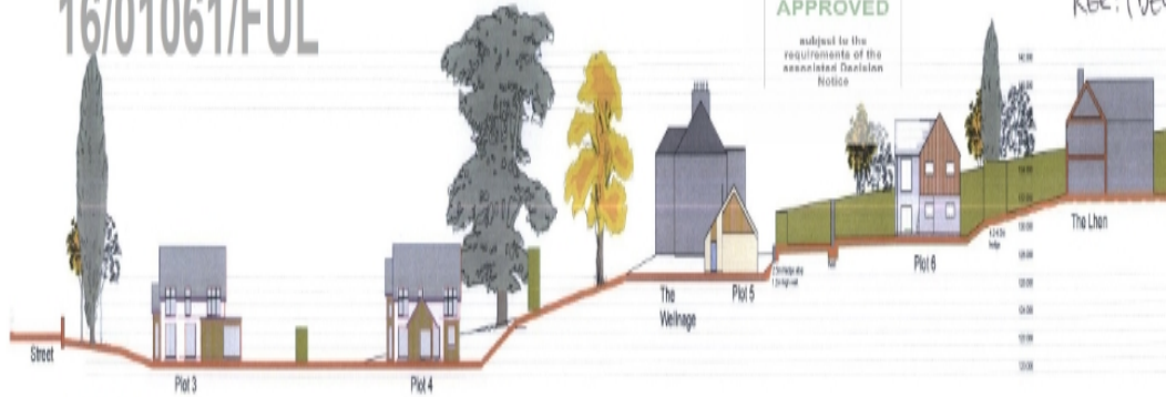
SECTION A - A 16/01061
